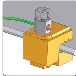
SI-2145A Structure Ground Clamp
