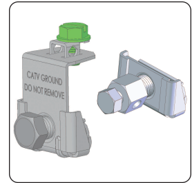
SI-2167GC / SI-2167C Meter Box Lip Mount Clamp
