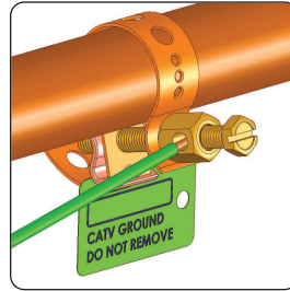
SI-0954-6 Ground Strap
