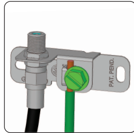
SI-GB-10 Single Ground Block
