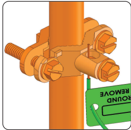
SI-5948G Water Pipe Clamp
