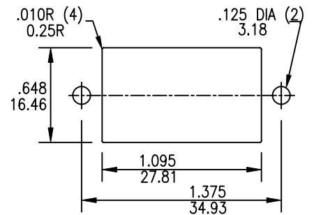
PANEL MOUNTING
