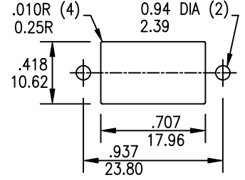
PANEL MOUNTING
