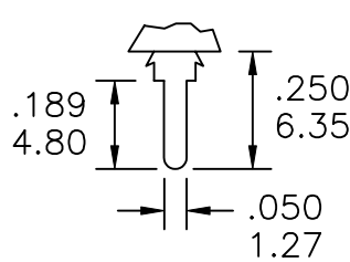
PC MOUNT
