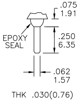
QUICK CONNECT
